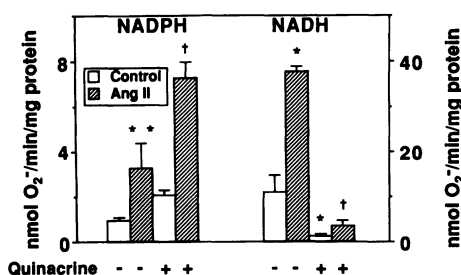
Fig 7. Bar graph showing the effect of quinacrine on NADPH and NADH oxidase activity in vascular smooth muscle cells. Vascular smooth muscle cells were exposed to angiotensin II (Ang II) or media alone (control) for 4 hours. Cells were then homogenized and added to a cuvette containing lucigenin alone (-) or lucigenin with 6 mmol/L quinacrine (+). Values for the NADPH assay are given on the left axis; values for the NADH assay are given on the right axis. Each bar represents the mean \pm SEM of the initial rate of enzyme activity for three (NADPH) or five (NADH) experiments. * P < .05 and ** P < .01 for Ang II vs control; † P < .05 for quinacrine+Ang II vs Ang II alone.
