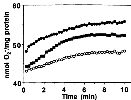
FIG 5. Graph showing stimulation of vascular smooth muscle cell NADPH oxidase by phosphatidic acid and arachidonic acid. Vascular smooth muscle cells were homogenized and added to a cuvette containing NADPH and lucigenin alone (○) or lucigenin and dioleoyl-phosphatidic acid (100 \mu g/mL) (■) or arachidonic acid (100 \mu mol/L) (●). Tracing is from one representative experiment repeated three to six times.
