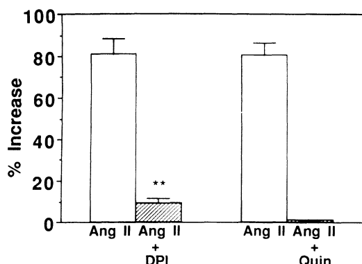
FIG 9. Bar graph showing attenuation of angiotensin II (Ang II)-induced hypertrophy by diphenylene iodinium (DPI) and quinacrine (Quin). Vascular smooth muscle cells were quiesced for 72 hours in 1% platelet-poor plasma, labeled with [ 3 H]leucine, and exposed to Ang II (100 nmol/L) in the presence or absence of DPI (10 μmol/L) or Quin (50 μmol/L) for 24 hours. [ 3 H]leucine incorporation was measured as described in "Materials and Methods." Data are expressed as the percent increase in [ 3 H]leucine incorporation induced by Ang II over the appropriate control. Each bar represents the mean of two (Quin) or three (DPI) experiments performed in triplicate. ** P <.01 for increase in the presence of inhibitor vs increase with Ang II alone. Quin was toxic to the cells.
