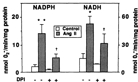
FIG 6. Bar graph showing the effect of diphenylene iodinium (DPI) on NADPH and NADH oxidase activity in vascular smooth muscle cells. Vascular smooth muscle cells were exposed to angiotensin II (Ang II) or media alone (control) for 4 hours. Cells were then homogenized and incubated with buffer (-) or 100 \mu mol/L DPI (+) for 5 minutes at room temperature immediately before the assay. Values for the NADPH assay are given on the left axis; values for the NADH assay are given on the right axis. Each bar represents the mean \pm SEM of the initial rate of enzyme activity for three (NADH) or four (NADPH) experiments. * P<.05 and ** P<.01 for Ang II vs control; † P<.05 for the effect of DPI on the Ang II signal vs the effect of Ang II alone.
