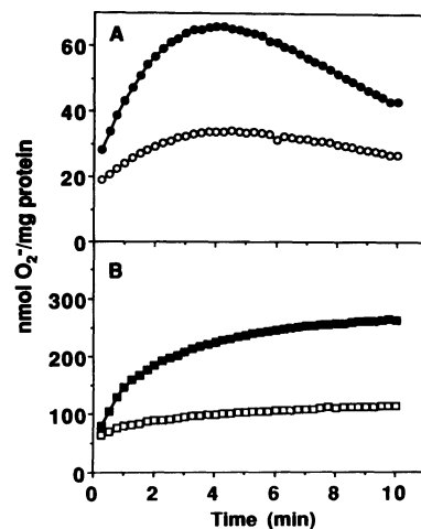
Fig 2. Graphs showing angiotensin II stimulation of NADPH and NADH oxidase activities. Vascular smooth muscle cells were exposed to angiotensin II (100 nmol/L) (filled symbols) or media alone (open symbols) for 4 hours, homogenized, and added to a cuvette containing dark-adapted lucigenin in a 50 mmol/L phosphate buffer. A, NADPH (100 \mu mol/L) was used as the substrate. B, NADH (100 \mu mol/L) was used as the substrate. Please note the difference in scale for the two graphs. Each tracing is from a representative experiment repeated 31 times for NADPH and 44 times for NADH. The mean initial rates are given in Table 1.
